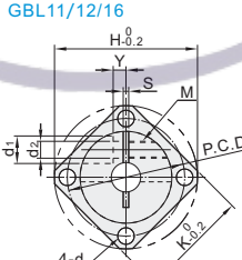
Square Flanged GBL11/12/16
