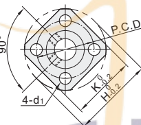
Square Flanged GAC11/12/16
