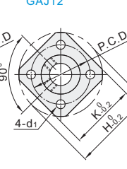
Square Flanged GAJ12
