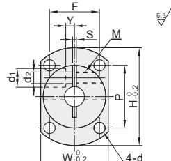
Compact Flanged GBJ21/22/26
