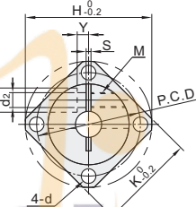
Square Flanged GBJ11/12/16
