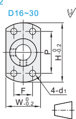
Compact Flanged GAJ21/22
