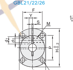
Compact Flanged GBL21/22/26
