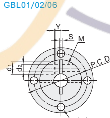
Round Flanged GBL01/02/06
