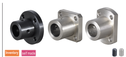
Compact Flanged GAC21/22/26/28
