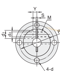
Round Flanged GBJ01/02/06
