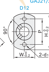
Compact Flanged GAJ21/22
