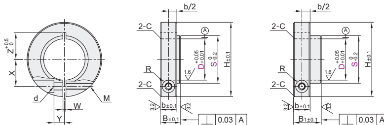
Short Shoulder FBH01/02/06
