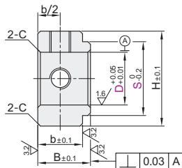
Short Shoulder FBC01/02/06/21/22
