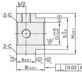
Long Shoulder FBC51/56/71/72
