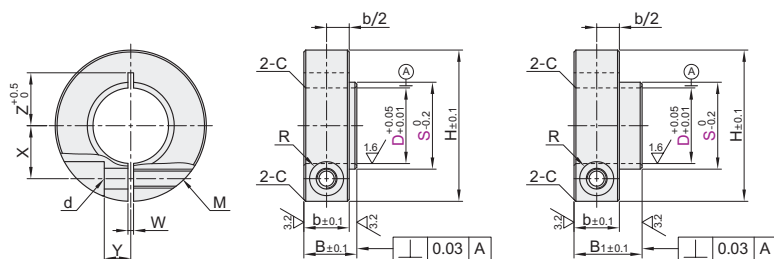
Short Shoulder FBG01/02/06/11/12
