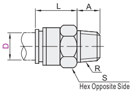
Straight XZC01
